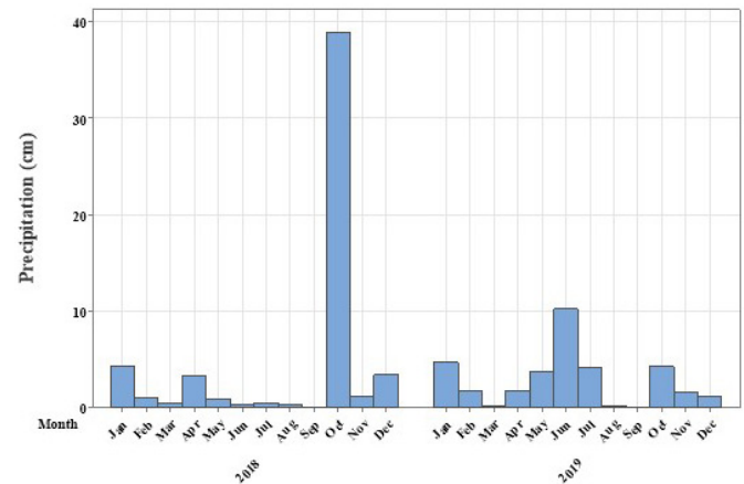
Fig. 3. Monthly precipitation (cm) totals for Laredo, Texas, USA during 2018 and 2019 (U.S. Climate Data 2020).
