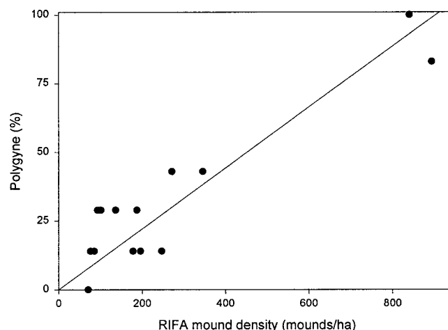
Fig. 3. Linear regression of RIFA mound densities against % occurrence of polygyny within sampling areas in Refugio County, Texas in 1998 and 1999 ( R^2 = 0.8392 , P < 0.0001 ).
