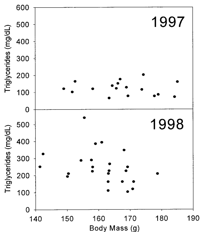
Fig. 1. Lack of linear relation between plasma triglycerides and body mass of northern bobwhites in 1997 and 1998, Refugio County, Texas (1997: R^2 = 0 , F_{1,15} = 0.20 , P = 0.660 ; 1998: R^2 = 0.12 , F_{1,21} = 2.87 , P = 0.105 ).
