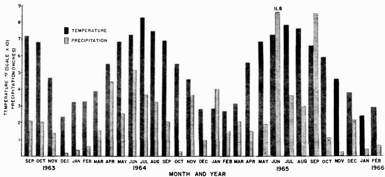
Figure 2. Temperature and precipitation corresponding with collection of bobwhite quail.
