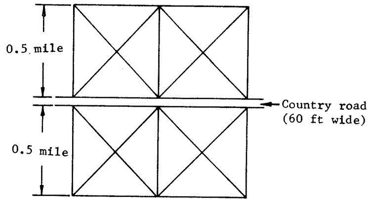
Figure 1. Diagram of diagonal lines used in calculating the interspersation index
