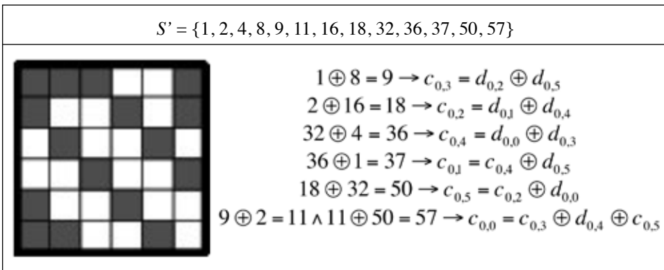
Figure 9: Example of set S' to schedule for a given bit-matrix.
