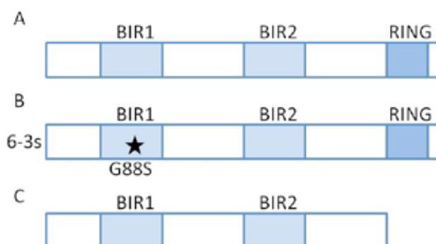
Figure 2. Protein structure of DIAP1.
