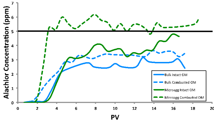
Fig. 3: In these herbicide transport curves, it seems that removing OM from the soil impedes the soils' ability to retain herbicide, and more herbicide is therefore released into the column effluent (asym p = 0.485 , xmid p = 0.114 , scale p = 0.457 ). Bulk soil seems to retain more herbicide than does the isolated microaggregate size fraction (asym p = 0.563 , xmid p = 0.651 , scale p = 0.657 ).
