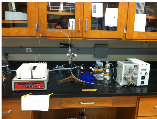
Fig. 2: This picture depicts the custom-designed soil column system used in this study. Depicted to the far right is the HPLC pump which actively pumped fluid through the Teflon and stainless steel tubing to the soil column. Fluid flowing out of the soil column was collected at regular intervals in quartz vials by a fraction collector system.
