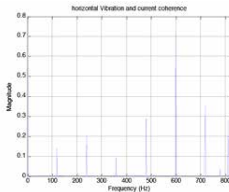
Figure 3.10: High coherence was found at some frequencies for horizontal vibrations and the motor current.
