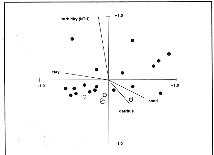
Figure 3. Ordination diagram based on canonical variates analysis (CVA) of sites where blackmouth shiners were found (open circles). The length and direction of the turbidity (NTU) vector suggests that water clarity had the greatest contribution in separating blackmouth shiner habitats from non-blackmouth shiner habitats.
