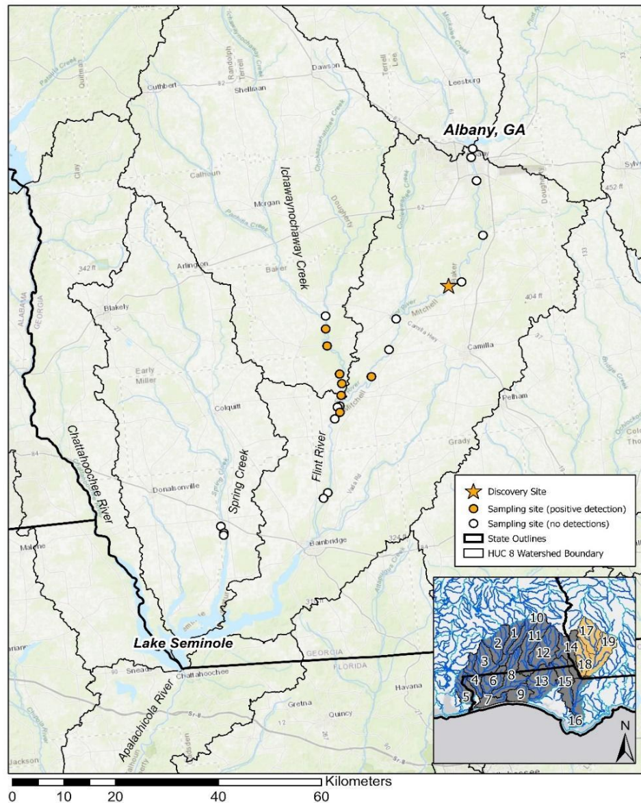
Figure 1. Sites where targeted searches for Ammocrypta were completed as part of this study. Lower inset shows watersheds included within the known range of A. bifascia , with watersheds sampled in Georgia highlighted. 1 = Patsaliga, 2 = Sepulga, 3 = lower Conecuh, 4 = Escambia, 5 = Perdido, 6 = Blackwater, 7 = Pensacola Bay, 8 = Yellow, 9 = Choctawhatchee Bay, 10 = upper Conecuh, 11 = Pea, 12 = upper Choctawhatchee, 13 = lower Choctawhatchee, 14 = lower Chattahoochee, 15 = Chipola, 16 = Apalachicola, 17 = Ichawaynochaway, 18 = Spring, 19 = lower Flint.
